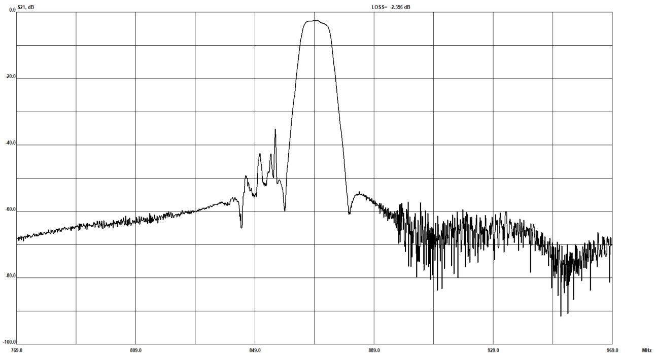
S21 response: (Span 200 MHz)
