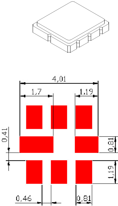
PCB Footprint
